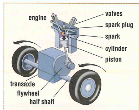
Transmitting power in a front-wheel drive vehicle
