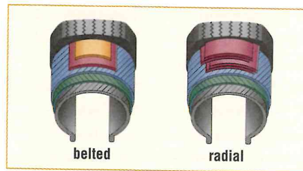
Tire construction
