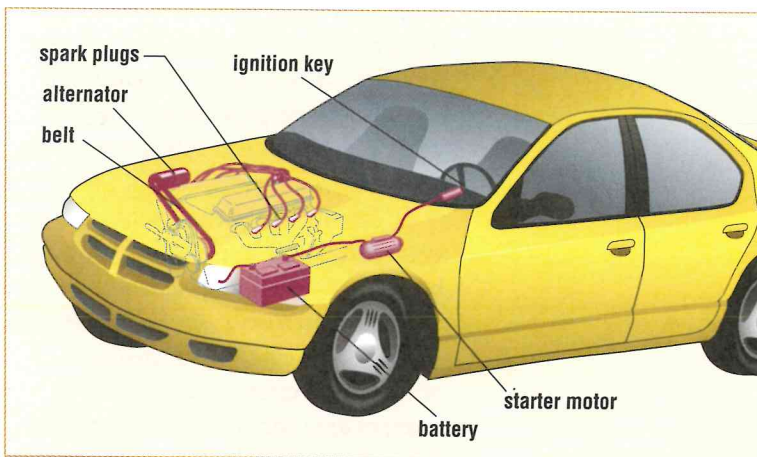
Ignition and electrical system
