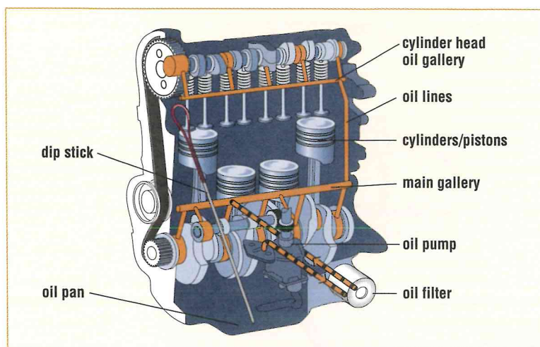
Lubrication system
