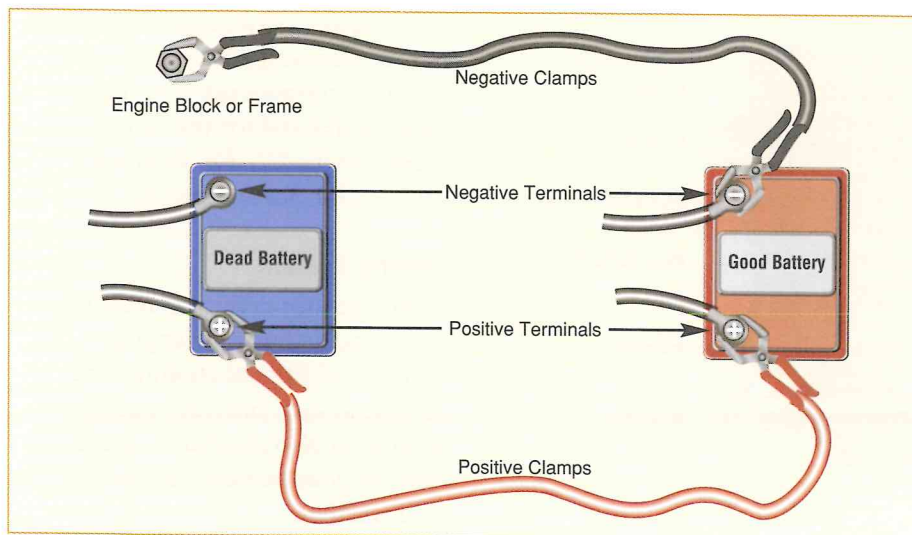
Jumper cable connections for jump-starting a vehicle
